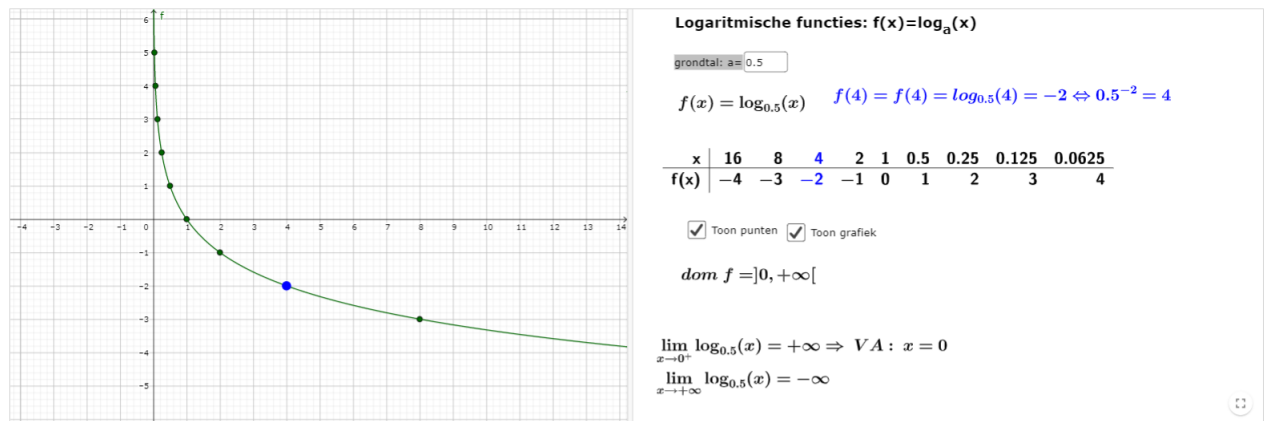
Figure 11: https://www.geogebra.org/m/ReNNrmut
