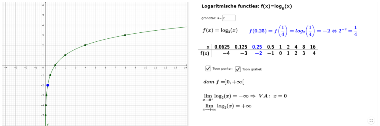
Figure 10: https://www.geogebra.org/m/ReNNrmut
