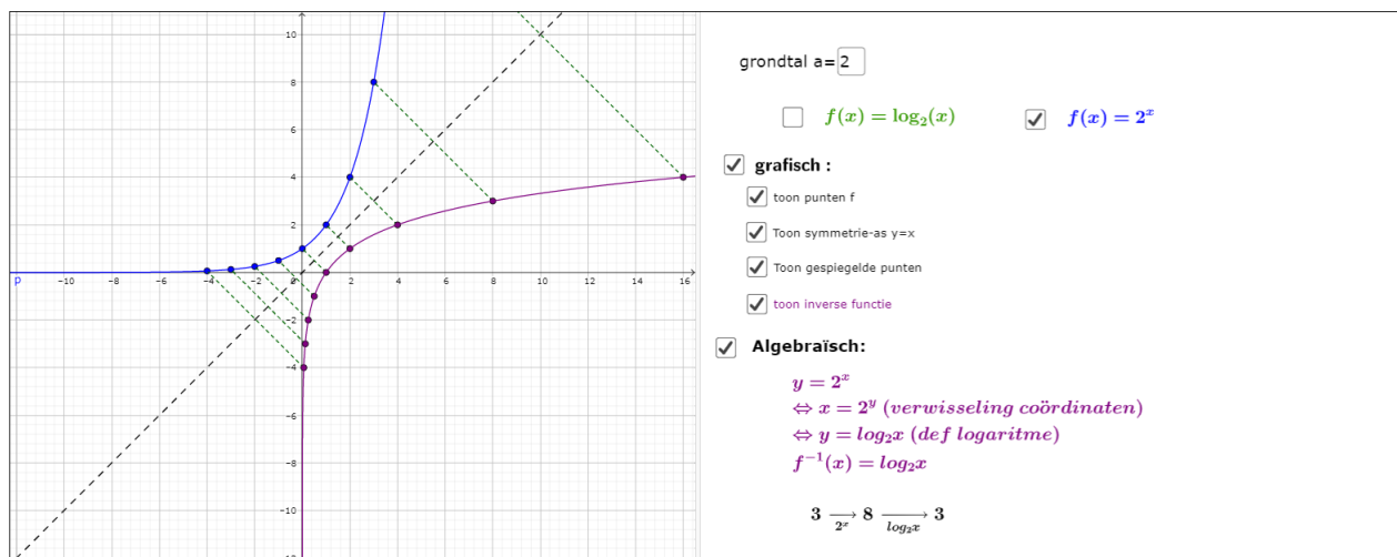
Figure 12: https://www.geogebra.org/m/YYevVAPy
