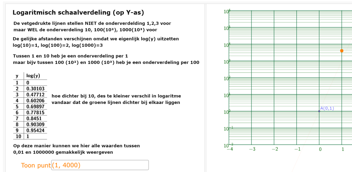
Figure 13: https://www.geogebra.org/m/gzggfr7h
