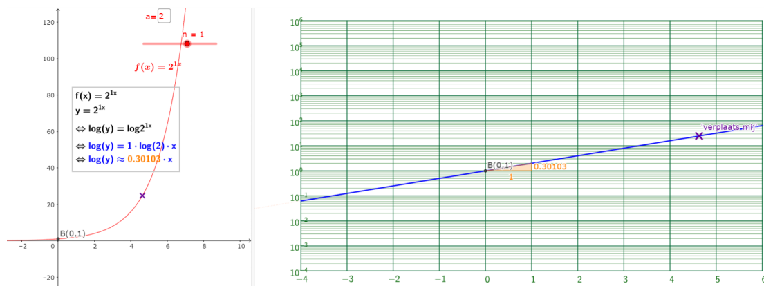
Figure 14: https://www.geogebra.org/m/gzggfr7h
