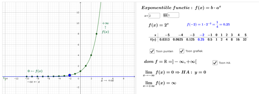
Figure 3: https://www.geogebra.org/m/Rb6qHp3z
