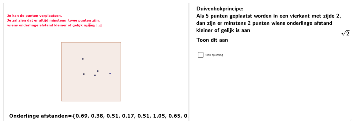
Figure 6: https://www.geogebra.org/m/sy2vvnnz
