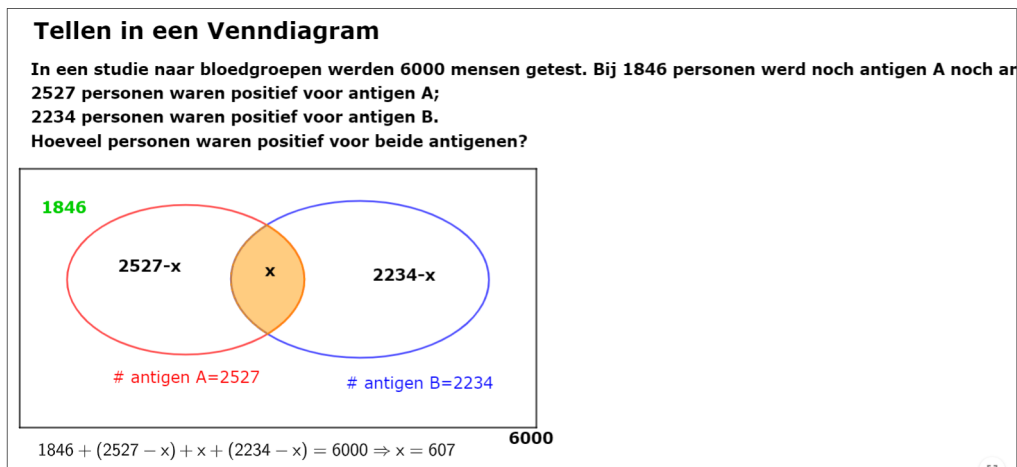
Figure 5: https://www.geogebra.org/m/m2h6yh47
