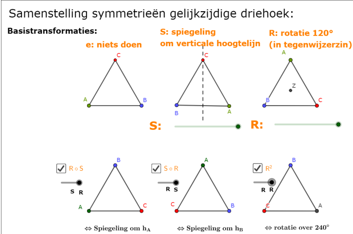
Figure 6: https://www.geogebra.org/m/qy4jbdnk
