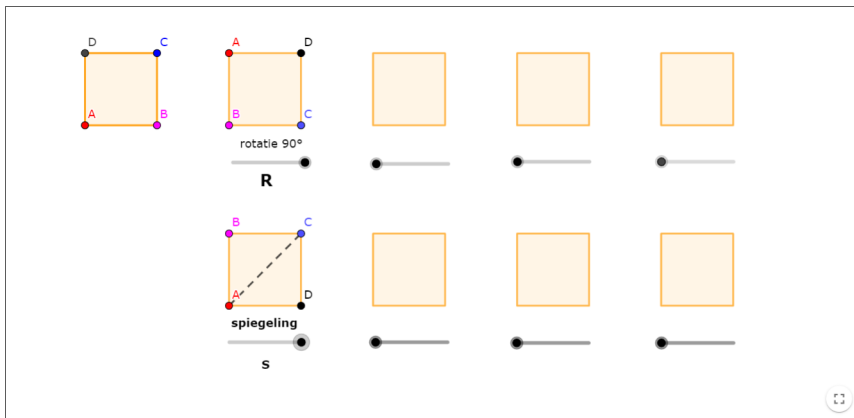
Figure 9: https://www.geogebra.org/m/fthabgvp
