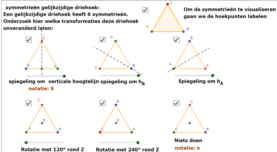
Figure 5: https://www.geogebra.org/m/qy4jbdnk
