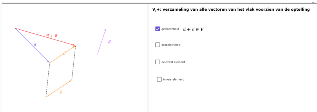
Figure 4: https://www.geogebra.org/m/x5n9emc3
