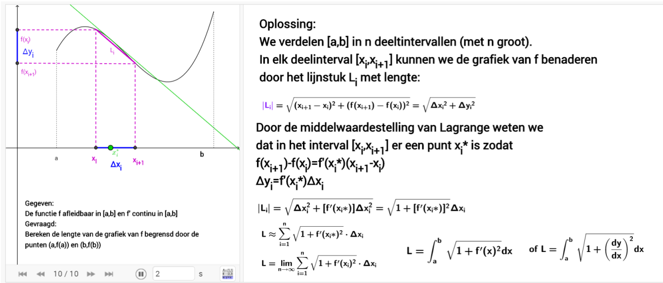
Figure 5: https://www.geogebra.org/m/C4h9qQaq
