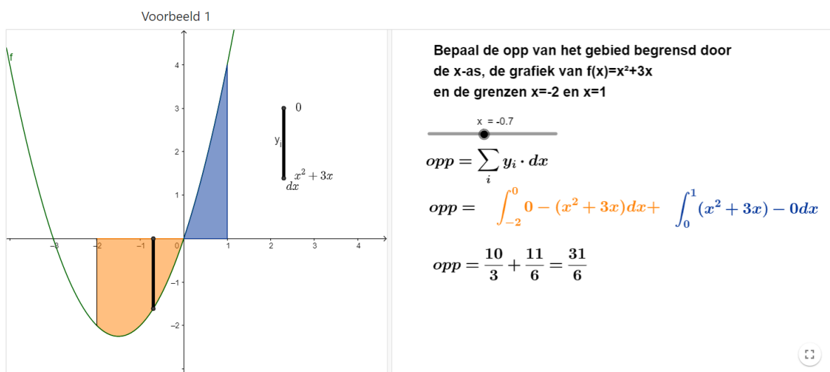
Figure 2: https://www.geogebra.org/m/QXvv6bTK
