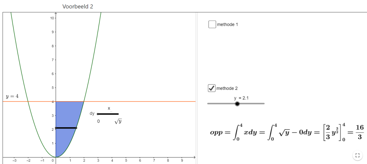
Figure 3: https://www.geogebra.org/m/QXvv6bTK
