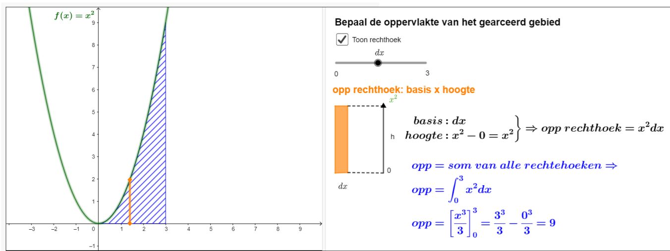
Figure 1: https://www.geogebra.org/m/QXvv6bTK
