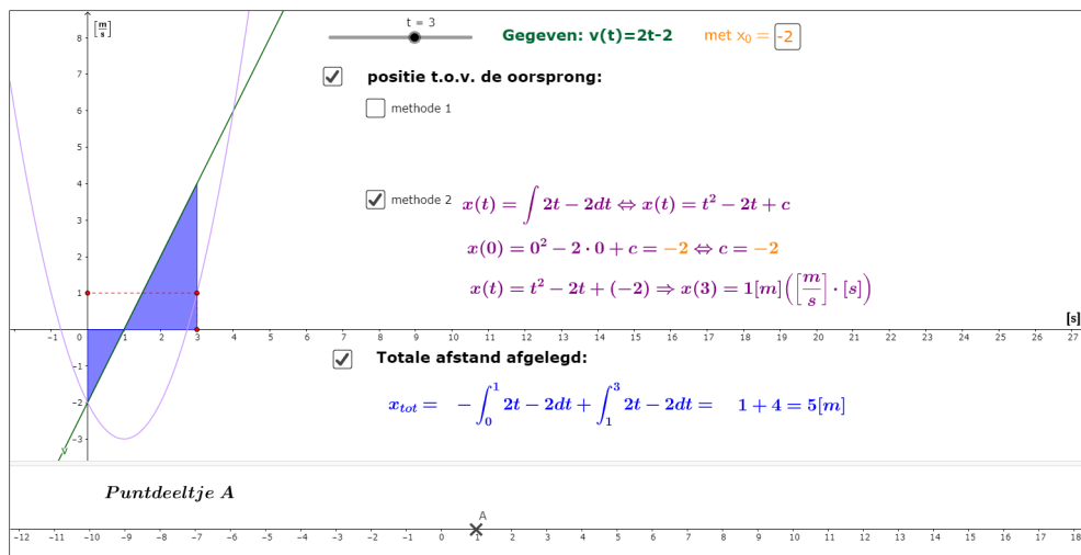
Figure 12: https://www.geogebra.org/m/vxxaKKUh
