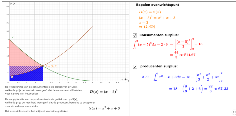
Figure 11: https://www.geogebra.org/m/d8kbjdv5
