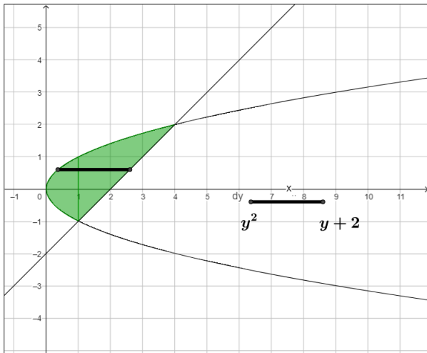
Figure 4: https://www.geogebra.org/m/QXvv6bTK
