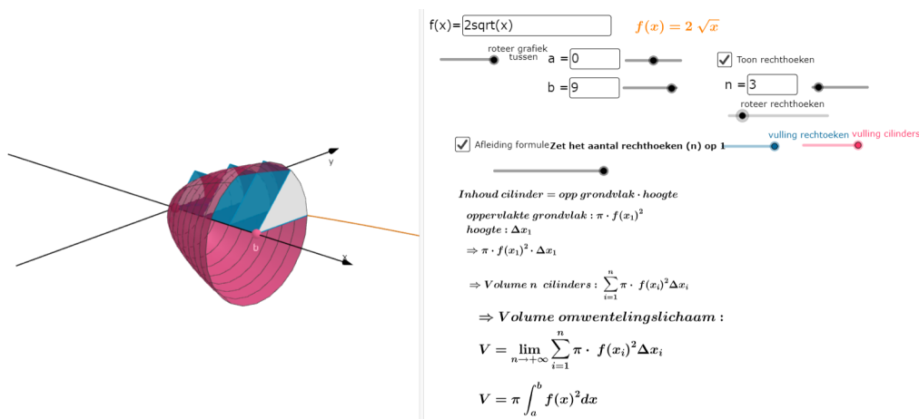
Figure 6: https://www.geogebra.org/m/b5DqDWuM
