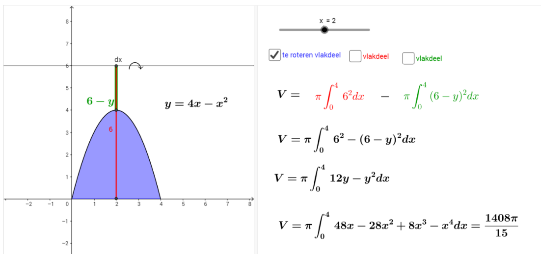
Figure 8: https://www.geogebra.org/m/b5DqDWuM
